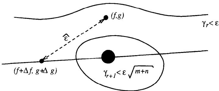
Fig. 1. The fat point represents the pairs with a GCD of degree \geq r + 2 , whereas the straight line includes the pairs corresponding to degree \geq r + 1 . The top curve is the boundary of neighborhood \gamma_r \leq \varepsilon and the closed curve is neighborhood \gamma_{r+1} \leq \varepsilon\sqrt{m+n} . Here, the degree of \hat{\varepsilon} -GCD may be superior to r + 1 , suggested by SVD with the given \varepsilon .
